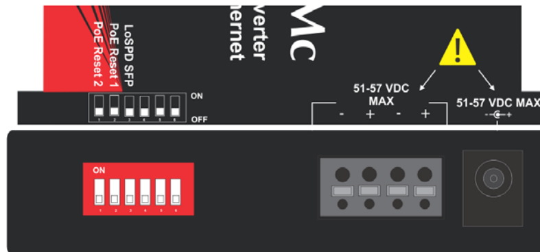
PoE+ Giga-MiniMc
