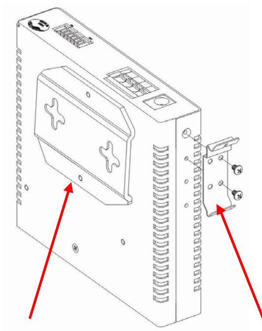
Wallmount Bracket
