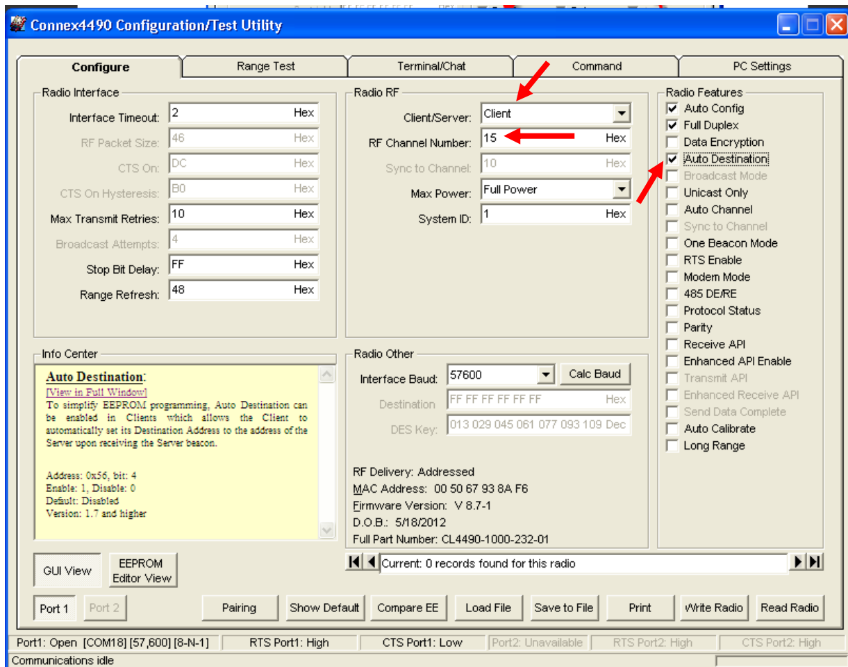
Figure 13: Client settings
