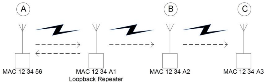
Figure 4: Loopback Repeater
