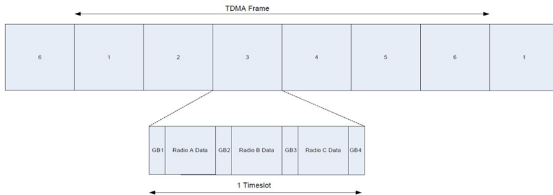
Figure 5: Quad Intervals
